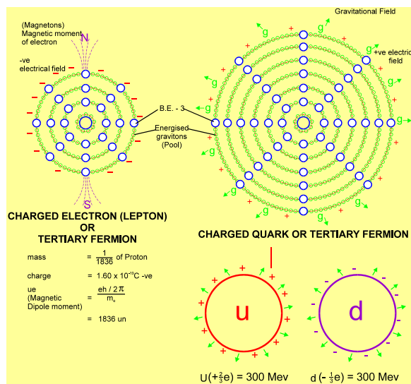
Fig 13 STRUCTURE OF QUARK AND ELELCTRON ( B.E. -3 or spin -3)
