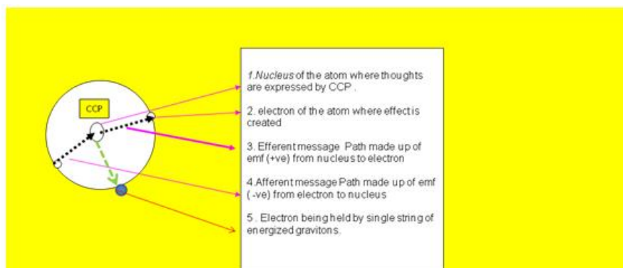
Fig 18 working of hydrogen atom – Divine MONB Theory underpins Photoelectric Effect
