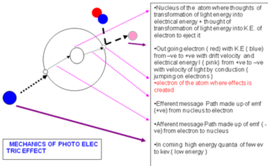
Figure 27 photo electric effect
