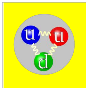
Fig 12 Wrong depiction of proton
