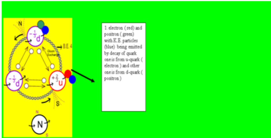
Fig 31 pair production at nucleons level
