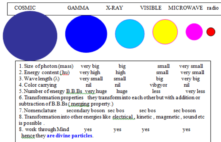
Fig17 Structure of gamma Rays, X rays , Visible Rays and Microwave
