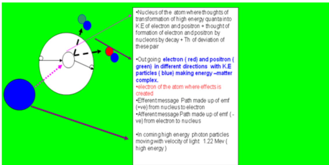
Fig 29 pair production
