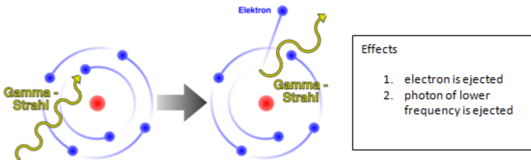
Fig 24 Compton effect ( wrong depiction ) [ 15]
