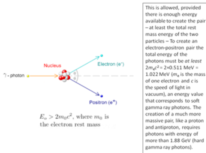
Fig 21 Pair production - Wrong Depiction [12]
