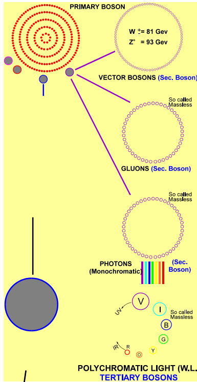
Fig 15 Structure of Polychromatic, Monochromatic, Gluons, Vector bosons and Higg's
