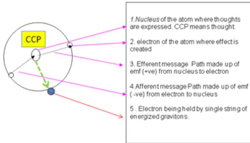
Fig 26 working of atom
