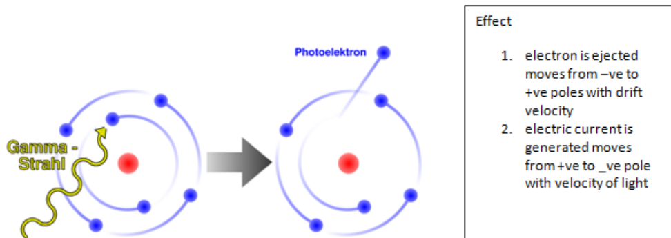
Fig 23 photo electric effect ( wrong depiction ) [14]
