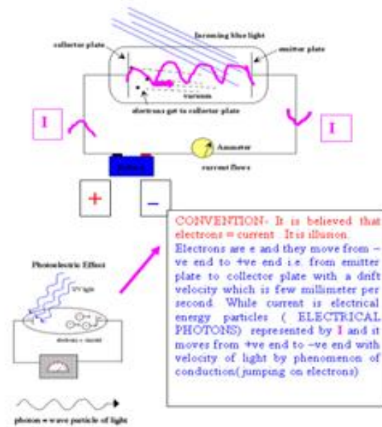
Figure 22 photoelectric effect [13]
