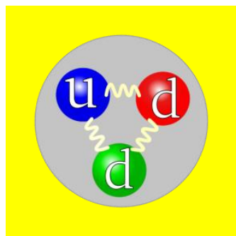
Fig 12.1 wrong depiction of neutron
