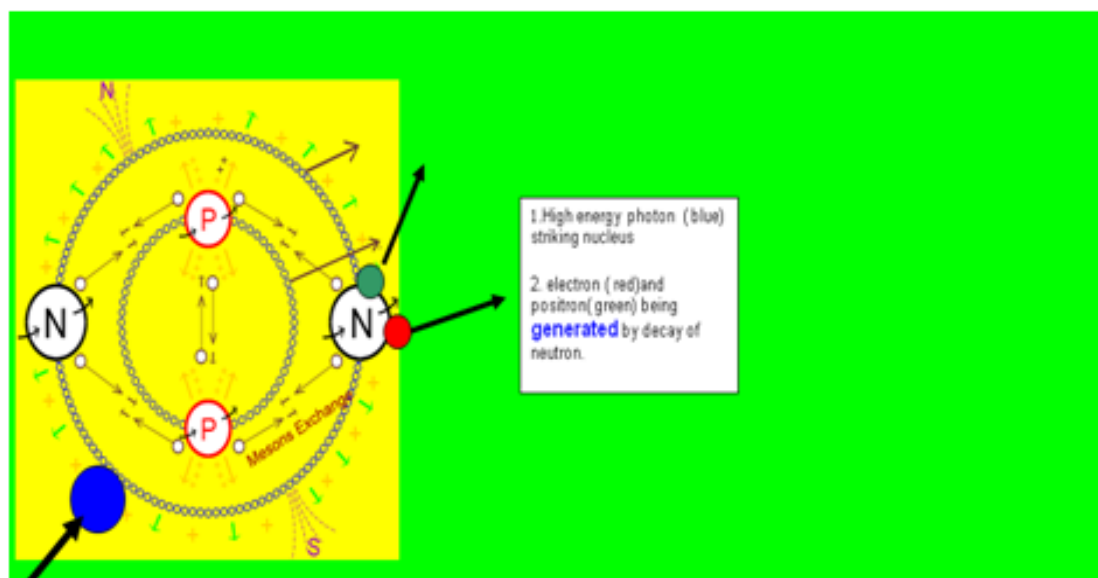
Fig 30 pair production at nucleus level
