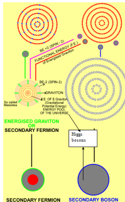
Fig 14 STRUCTURE OF ENERGISED GRAVITONS ( Binding energy -2) or( spin -2) AND SCONDARY BOSONS - HIGG'S (BINDING ENERGY or B.E.)
