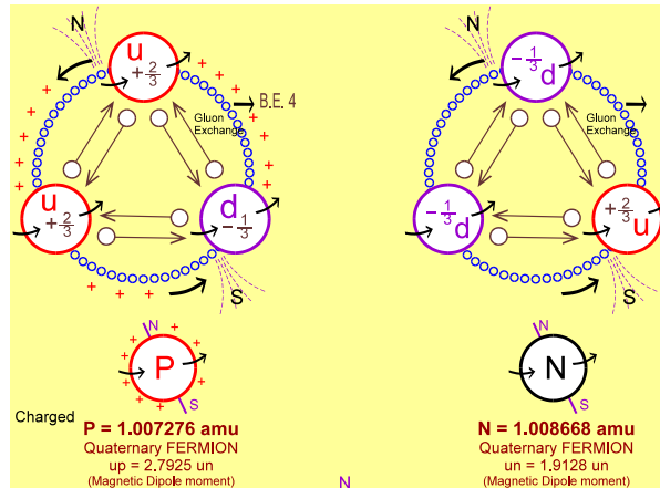
Fig 12.2 STRUCTURE OF PROTON AND NEUTRON- Right Depiction ( B.E.-4 or spin -4)
