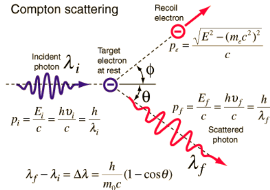
Fig 19 Compton effect - Wrong Depiction [10]
