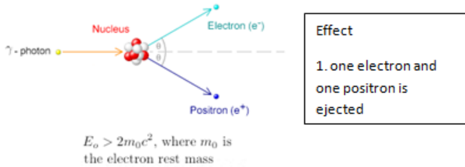
Fig 25 pair production ( wrong depiction ) [16]
