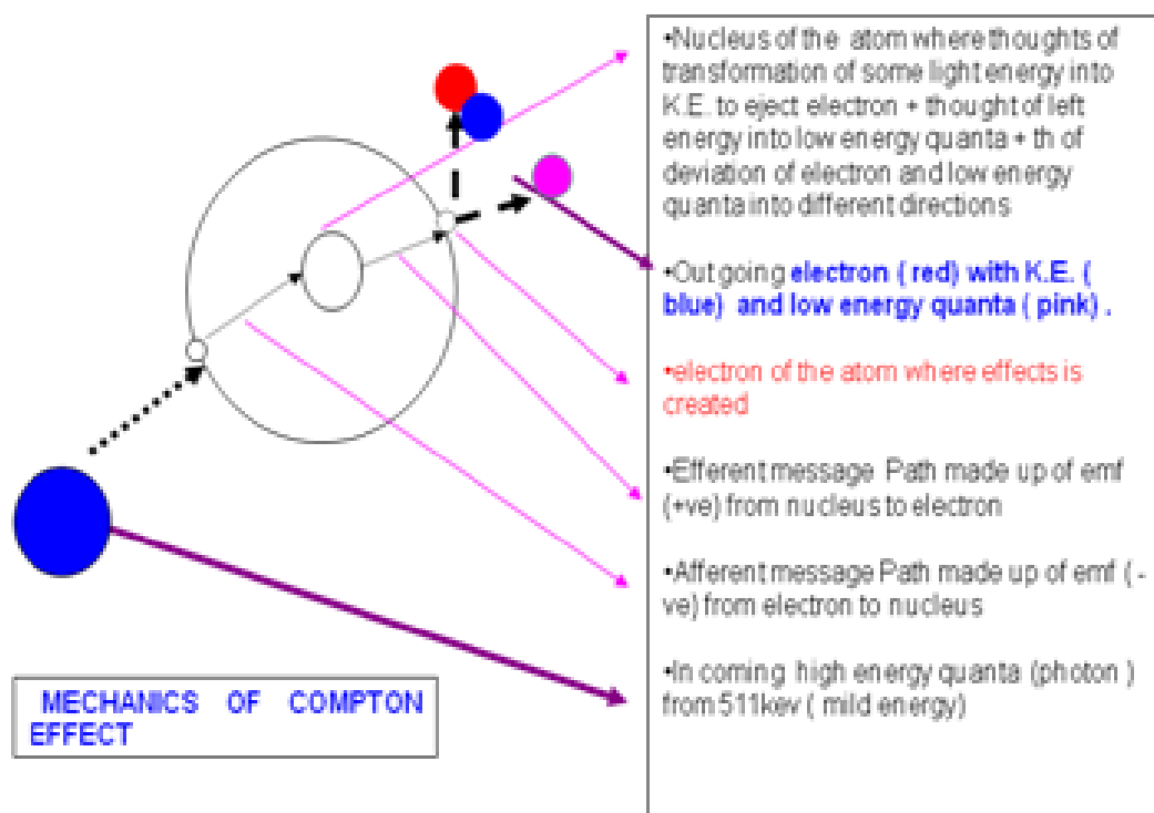
Figure 28 Compton effect
