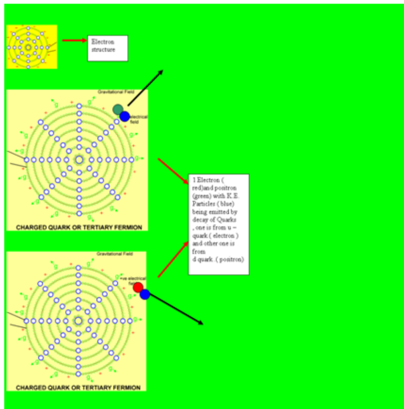
Fig 32 pair production at quark level
